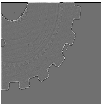
5x5 Mexican Hat - Laplacian of Gaussian
